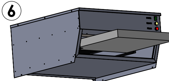
Slide out large fine filter from stack, Inspect every 2 months or 500 hours of use Replace every 6 months or 1500 hours of use
