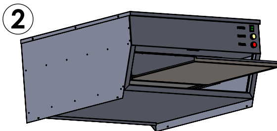
Slide out Tray and replace lower layer of filter media every 2 months or 500 hours of use Replace upper layer of media every 6 months or 1500 hours of use
